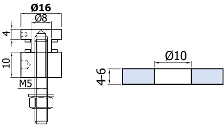
PG-21 e▶ 1.83 • Daugybinis tarpiklis 8 mm, skirtas PG-20. • Distance rings 8 mm for PG-20.
