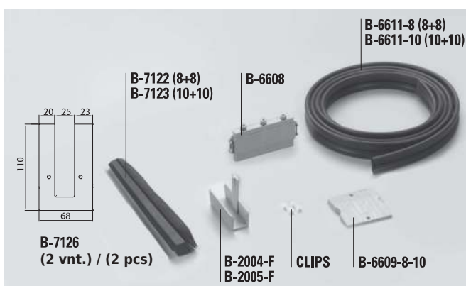
B-SET-7120-8 • Stiklui / For glass: 8+8
