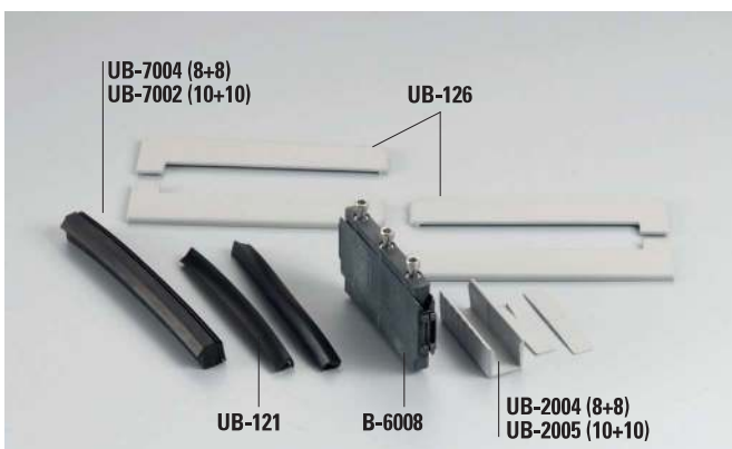
UB-SET-120-8 Stiklui: 8+8 UB-SET-120-10 Stiklui: 10+10 €▶H.141 UB-SET-120-8 For glass: 8+8 UB-SET-120-10 For glass: 10+10
